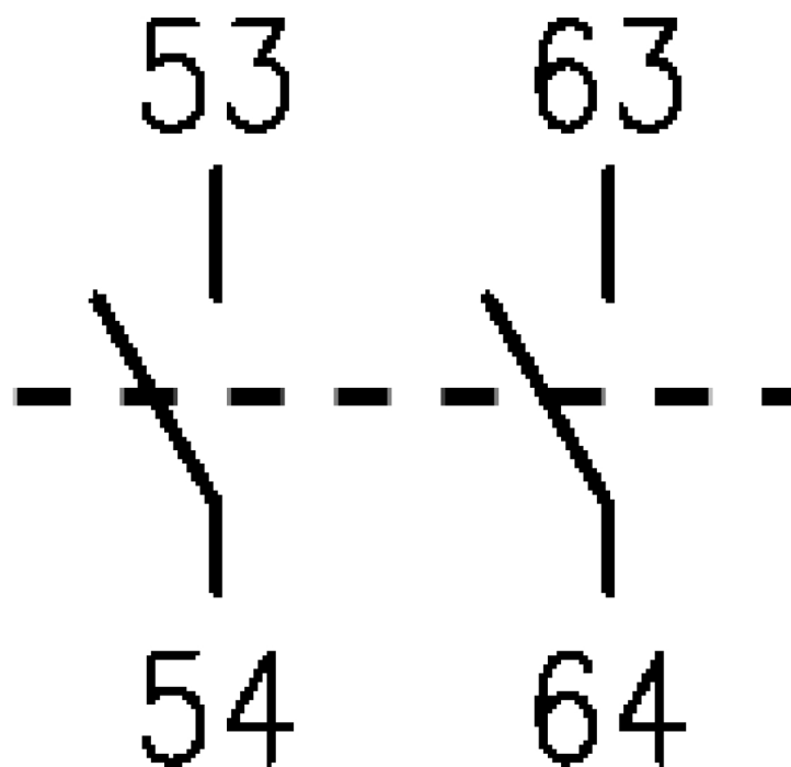
Connection / Wiring Diagram
